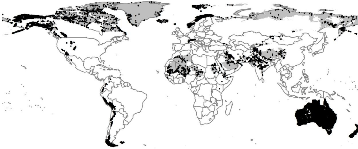
Figure 2. Randomly selected background grid cells used in the modelling of Faxonius rusticus , mapped as points. Points are sampled from the native range, a small buffer around non-native occurrences and from areas expected to be highly unsuitable for the species (grey background region), and weighted by a proxy for recording effort (Figure 1b).
